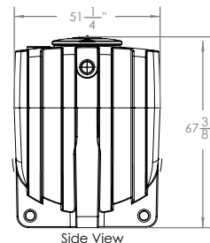
Baffle and Filter Customizable to create 2-3 chambers
